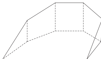
FIGURE 3. A polytope combinatorially equivalent to the shell S_7 .
