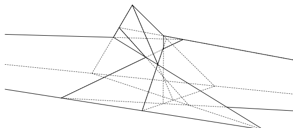
FIGURE 5. An arrangement formed by 6 planes maximizing the average diameter.
