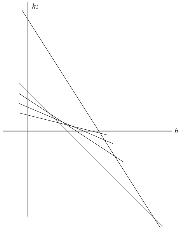
FIGURE 1. An arrangement combinatorially equivalent to \mathcal{A}_{2,7}^o .
