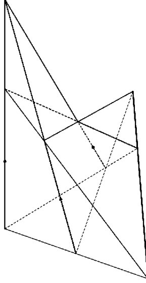
FIGURE 6. An arrangement combinatorially equivalent to \mathcal{A}_{3,5} .
