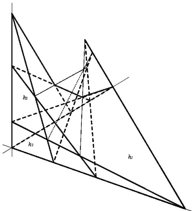
FIGURE 4. An arrangement combinatorially equivalent to \mathcal{A}_{3,6}^* .
